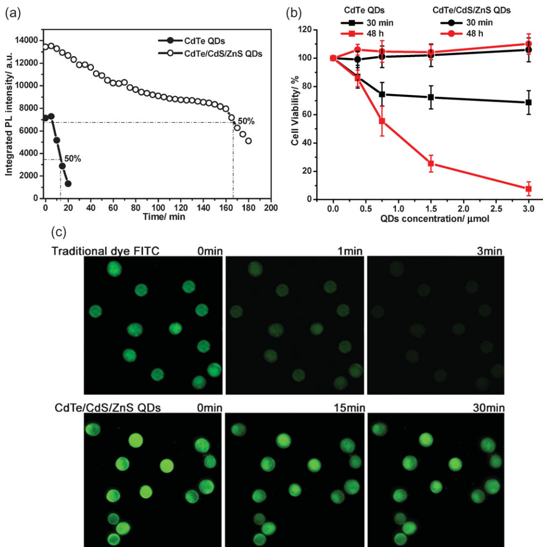
Figure 5. a) Evolution of the integrated PL intensity of oxygen-saturated solutions of CdTe and the CdTe/CdS/ZnS QDs under irradiation (Xenon lamp, 365 nm, 450 W). b) Cytotoxicity of different concentrations of CdTe and CdTe/CdS/ZnS QDs in K562 cells. c) Comparison of the photostability of fluorescein isothiocyanate (FITC) and CdTe/CdS/ZnS QDs upon staining of ethanol-fixed K562 cells.
