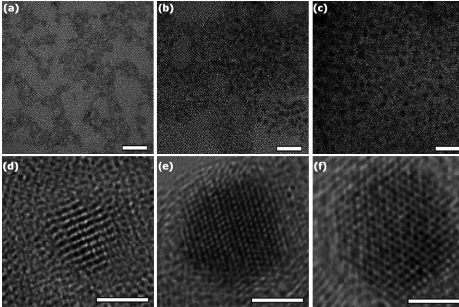
Figure 3. Transmission electron microscopy (TEM, top) and high-resolution (HR) TEM (bottom) images of a), d) CdTe core QDs; b), e) CdTe/CdS core-shell QDs; and c), f) CdTe/CdS/ZnS core-shell-shell QDs synthesized using microwave irradiation. Scale bars are 20 nm (a–c) and 2 nm (d–f), respectively.
