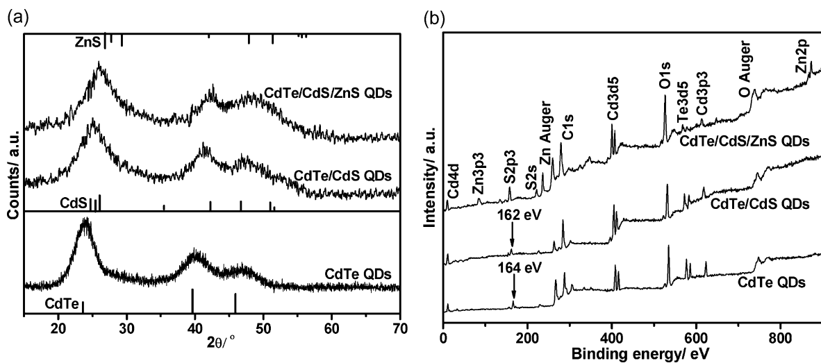
Figure 4. a) Powder X-ray diffraction (XRD) patterns of CdTe core QDs, CdTe/CdS core-shell QDs, and corresponding CdTe/CdS/ZnS core-shell-shell QDs. Standard diffraction lines of cubic CdTe, cubic CdS, and cubic ZnS are shown for comparison. b) X-ray photoelectron spectra (XPS) of the same materials.
