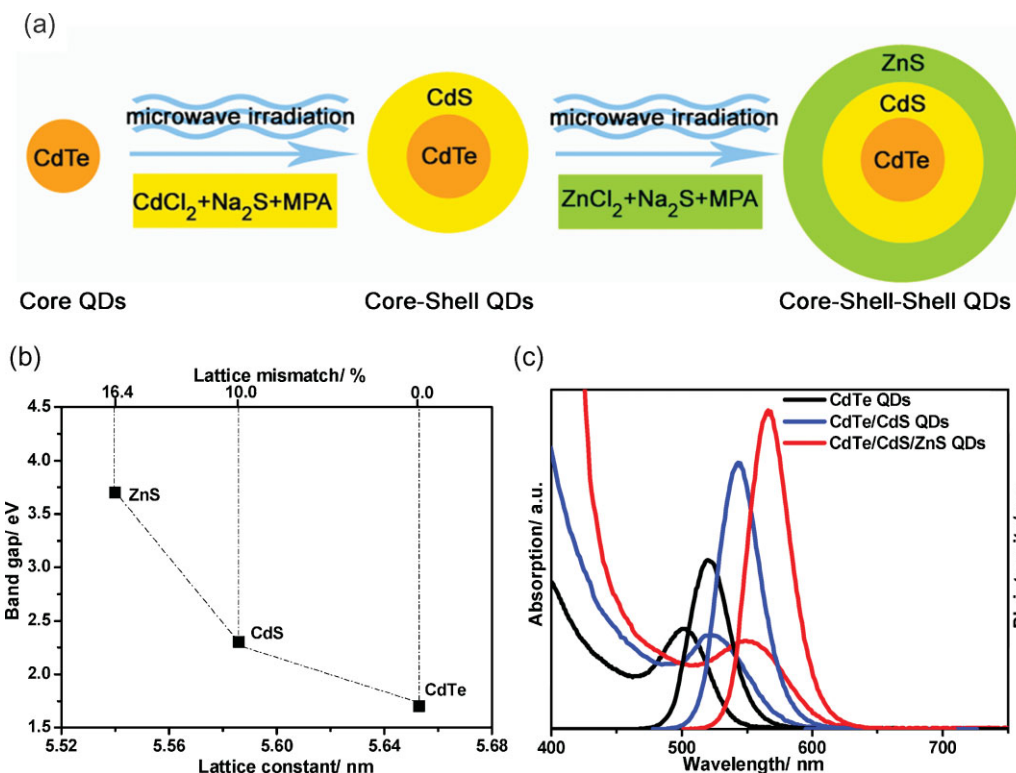
Figure 1. a) Schematic illustration of microwave (MW)-assisted synthesis of water-dispersed CdTe/CdS/ZnS core-shell-shell (CSS) quantum dots (QDs). b) Interrelationship between band gap energy, lattice constant, and lattice mismatch of bulk CdTe, CdS, and ZnS. Herein, lattice mismatch refers to the mismatch compared to CdTe. c) Representative absorption and photoluminescence (PL) spectra of CdTe core QDs (photoluminescence quantum yield (PLQY) ~30%), CdTe/CdS core-shell QDs (PLQY ~65%), and corresponding CdTe/CdS/ZnS core-shell-shell QDs (PLQY ~80%) prepared at 100 °C and 1 min MW irradiation, 100 °/5 min, and 60 °C/5 min, respectively.
