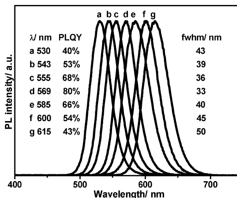
Figure 2. PL spectra of synthesized CdTe/CdS/ZnS core-shell-shell QDs with a series of maximum emission wavelengths. Related PLQY and full width at half maximum (fwhm) values are presented.
