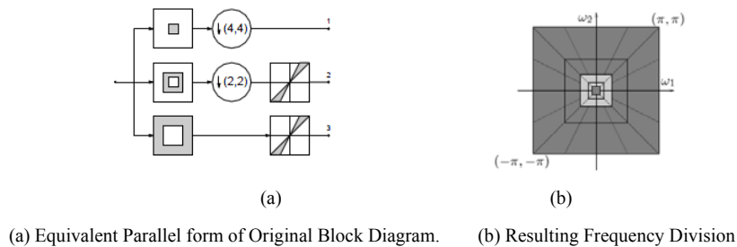
Fig.1 The Original Contourlet Transform
