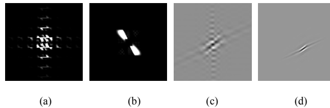
Fig. 4 Comparison on Basis image of the Original Contourlet and SFLCT. (a) and (b) Basis Images of Original Contourlet and Sharp Frequency Localized Contourlet in Frequency Domain. (c) and (d) Basis Image of the Two Transforms in Spatial Domain.
