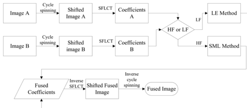
Fig. 5 Framework of Image Fusion Method in Our Paper.
