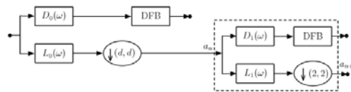
Fig. 3 The Block Diagram of SF.
