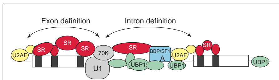
Fig. 4. Intron and exon definition models for pre-mRNA recognition. The model is based on information derived from both metazoan and plant splicing. Interactions of U1 small nuclear ribonucleoprotein (snRNP; labelled U1) with the 5' splice site (ss), and U2AF (yellow) with the region between the branch point and the 3' ss are early events of splice-site recognition taking place within the E complex. Uridylate-specific RNA-binding hnRNP-like proteins represented by green ovals, together with SR proteins (red ovals) bound to the putative exonic splicing enhancers assist in the binding of U1 snRNP and U2AF to the pre-mRNA and in establishing cross-intron and cross-exon contacts between the splice sites. The branch point bridging protein (BBP/SF1; blue) that interacts with the branch point (A), helps to position U2AF 65 to the polypyrimidine tract through cross-intron interaction 1,3 . Because the gene encoding BBP/SF1-like protein is present in Arabidopsis (AB023044), this interaction is likely to occur in the plant E complex as well. All components indicated, except exonic splicing enhancers (ESEs; black boxes), have been identified in plants. U1-70K depicted in grey.
